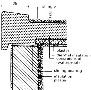
1 Waterproof concrete roof (Woermann roof)
